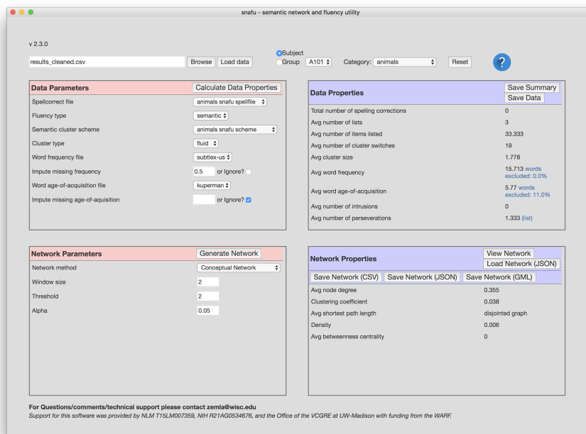
Fig. 2 The GUI allows you to see at a glance many properties of the fluency, as well as properties of a network generated from the data.
